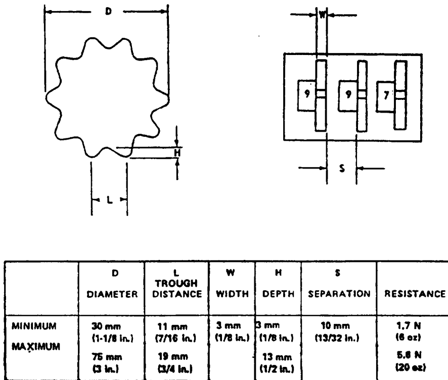
FIGURE 6. Discrete thumbwheel control
