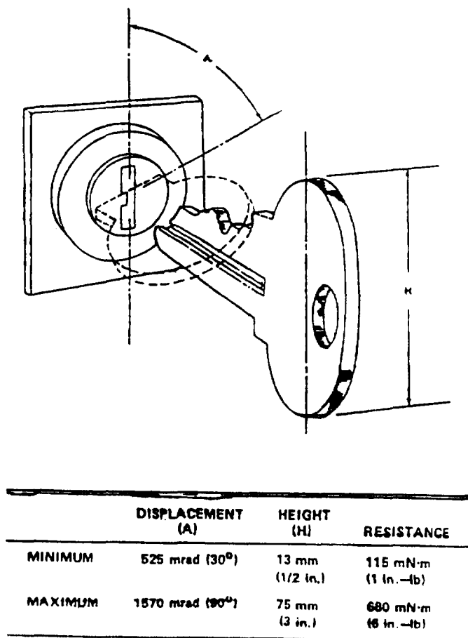
FIGURE 5. Key-operated switch
