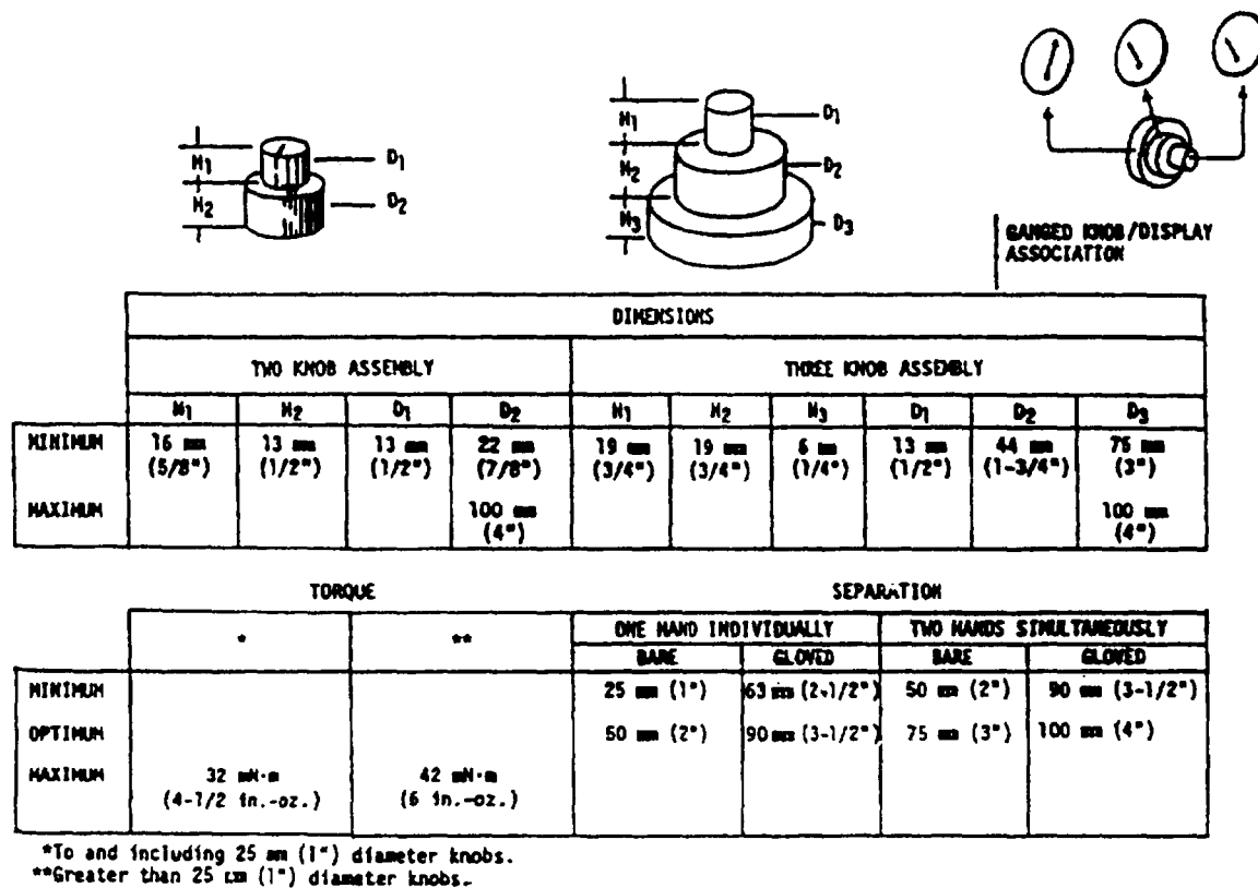
FIGURE 8. Ganged knobs
