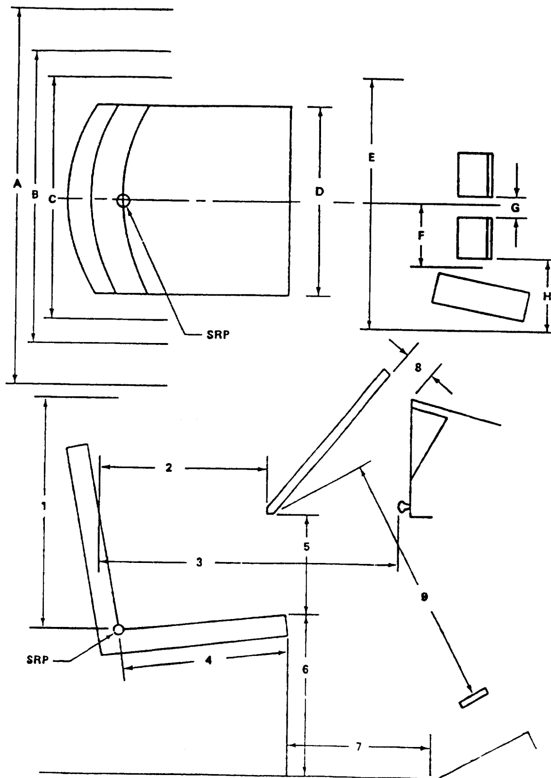
FIGURE 51. Recommended clearances around equipment
