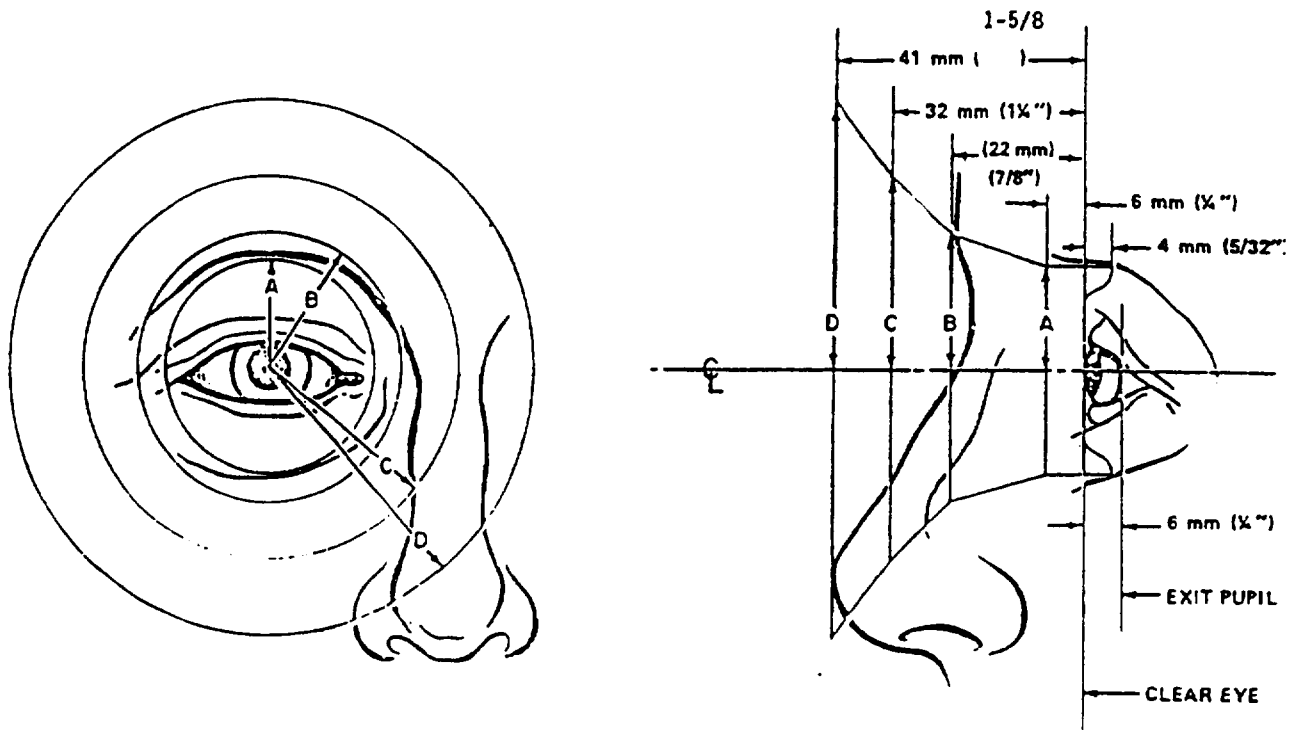
FIGURE 49. Anatomical limits on axially symmetrical ocular metal parts
