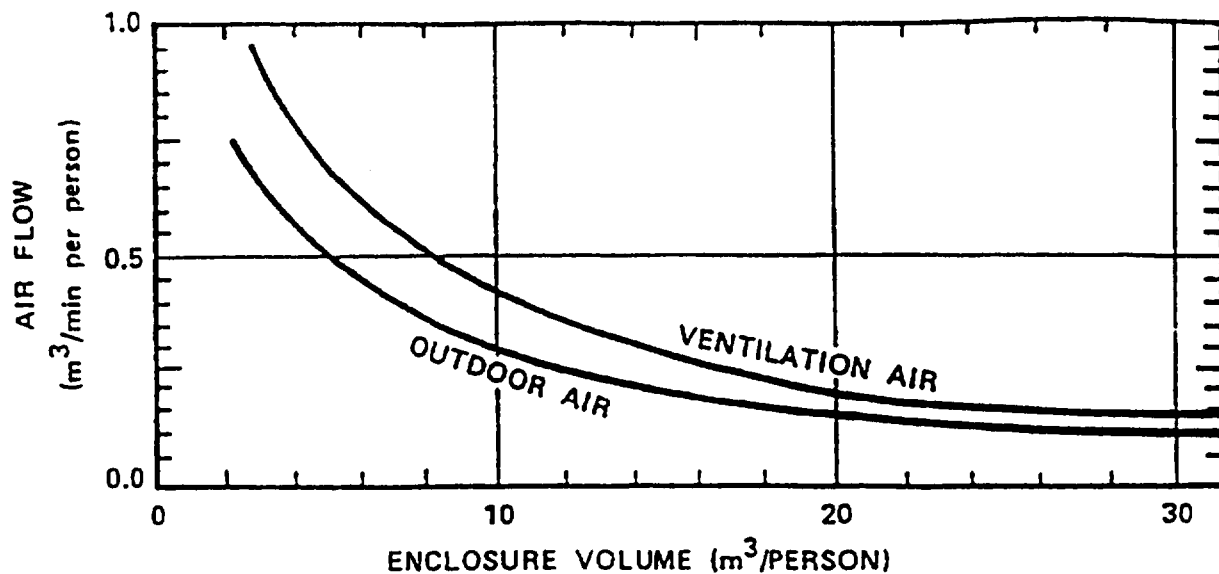
FIGURE 39. Ventilation requirements
