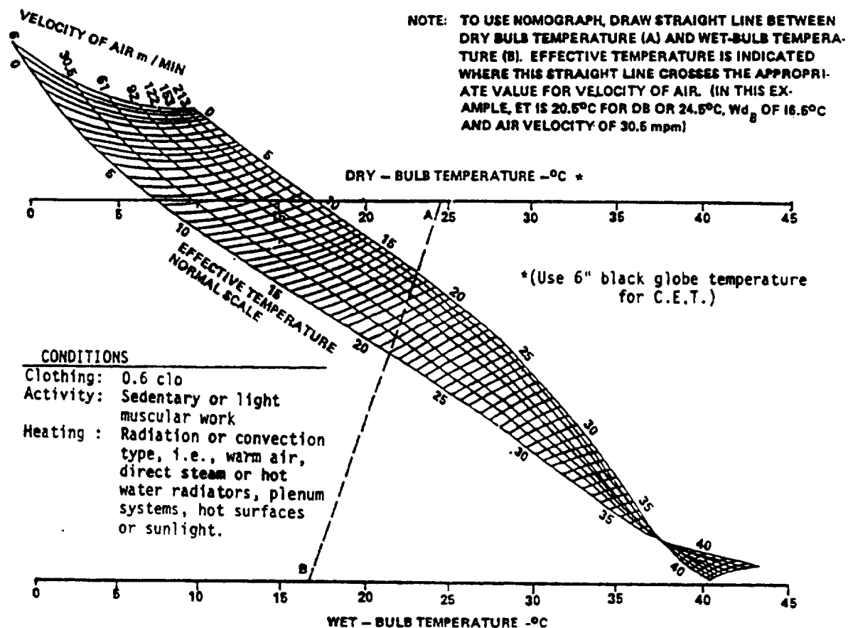
FIGURE 38. Effective temperature (E.T.) or corrected effective temperature (C.E.T.)
