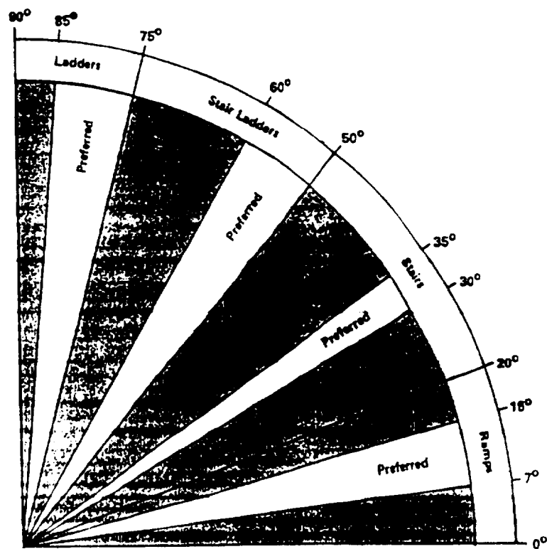
FIGURE 33. Type of structure in relation to angle of ascent
