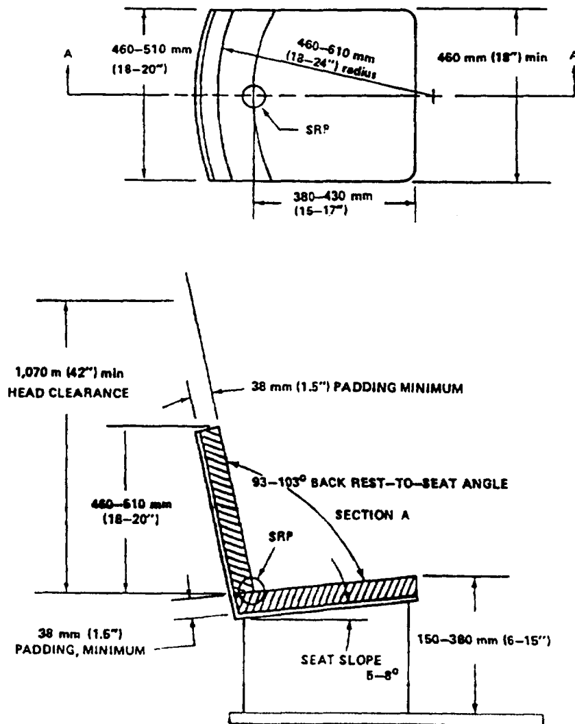
FIGURE 50. Dimensions for vehicle operator's seat
