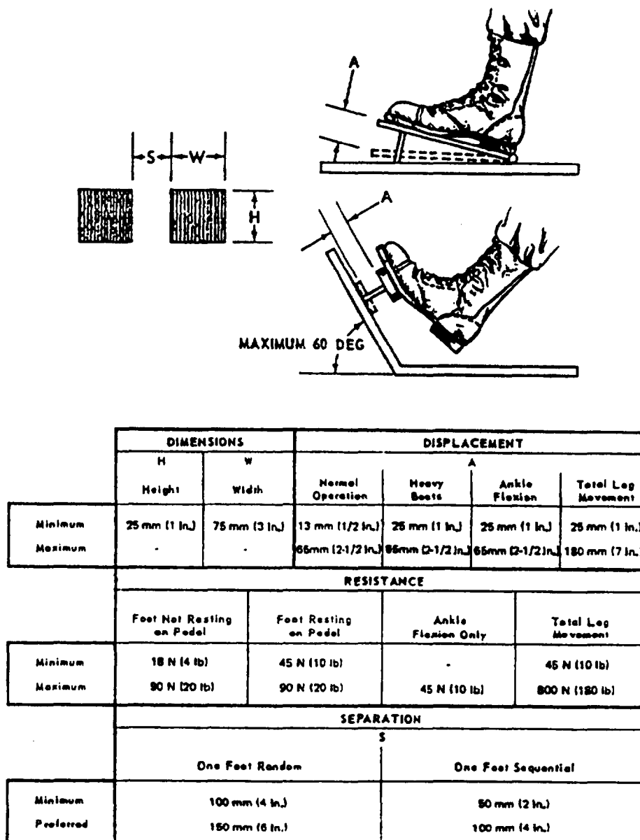
FIGURE 20. Pedals
